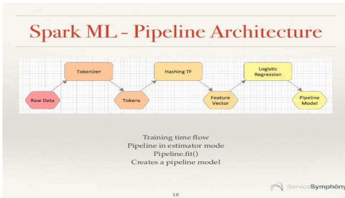
Fig 4: Spark Architecture:
