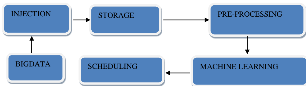
Fig 3: Preprocessing Pipeline:
