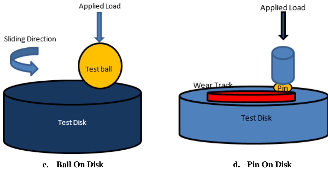
Fig 3. Schematic diagrams of Tribological tests.
