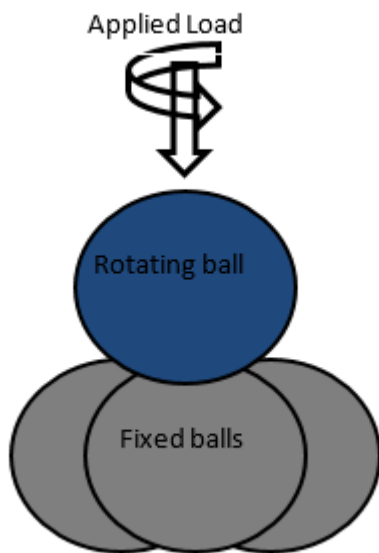
a. Four Ball tester
