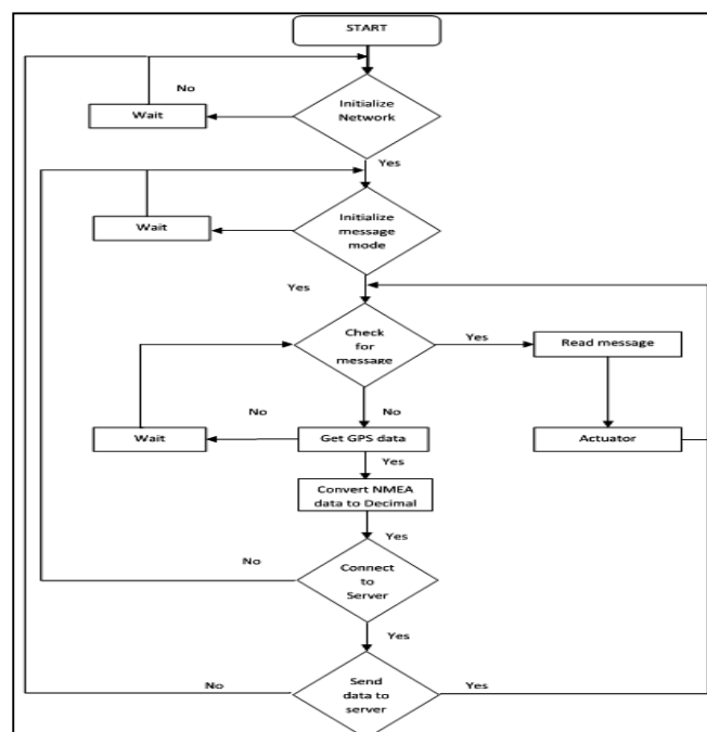
Fig 3. Hardware flow chart (overall)
