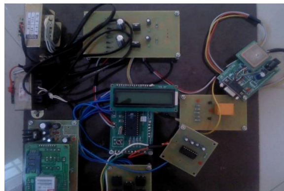
Fig 2 Vehicle Module
