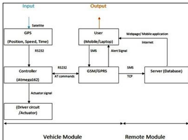
Fig 1 Vehicle Monitoring with Remote Access
