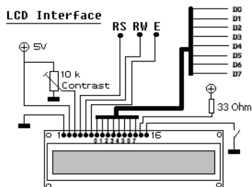
FIG. 5. LCD INTERFACE
