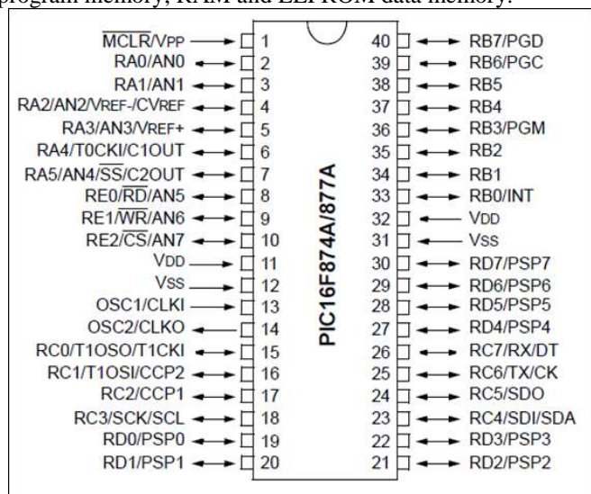
FIG. 1. PIN LAYOUT OF PIC16F877A
