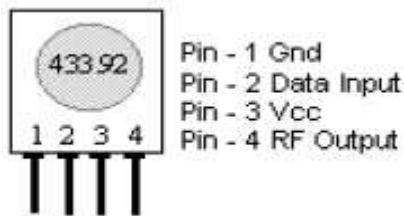
FIG. 6. TWS-434 PIN DIAGRAM
