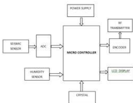
FIG. 3. BLOCK DIAGRAM OF NODE 1
