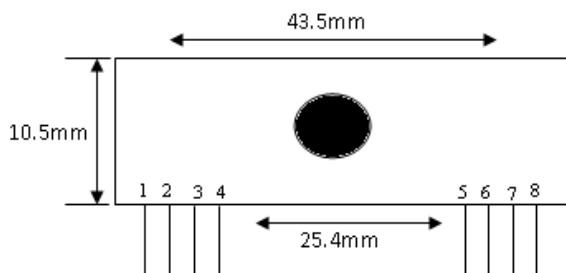
FIG. 7. RWS-434 PIN DIAGRAM
