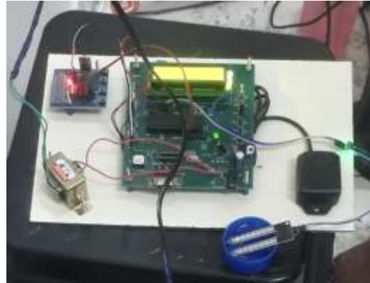
FIG. 12. FLOOD MONITORING ELECTRICAL CIRCUIT NODE 1
