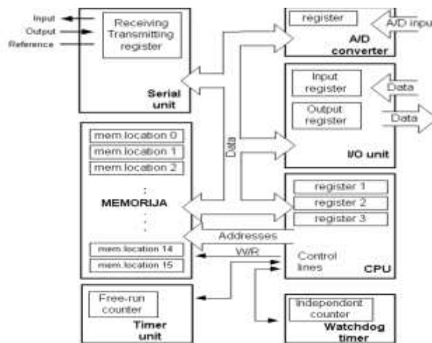
FIG. 2. BLOCK REPRESENTATION OF THE MICROCONTROLLER
