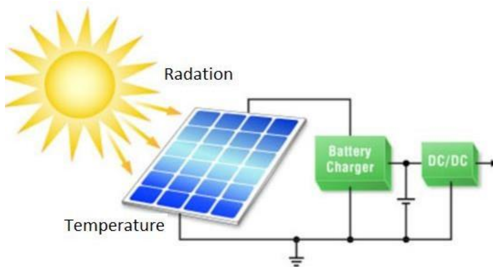
Figure (4) shows a solar system without a booster system
