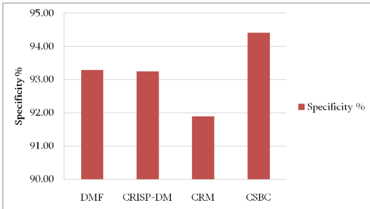
Fig. 10: Specificity
