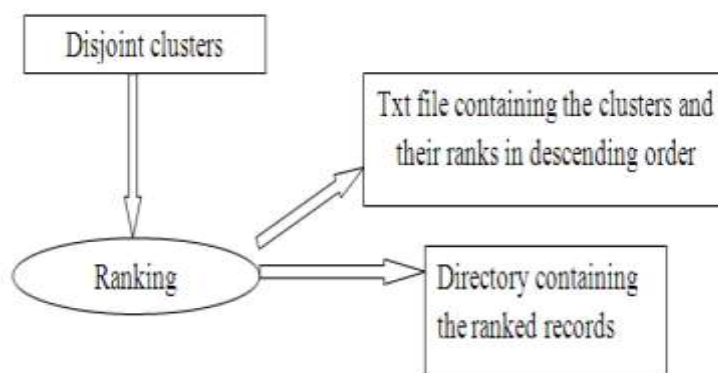
Fig. 4 detailed Ranking
