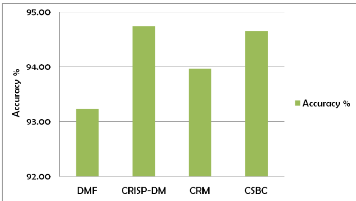
Fig. 9: Accuracy
